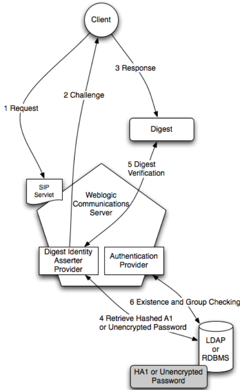
Figure 2-1 Digest Authentication in Oracle Communications Converged Application Server
